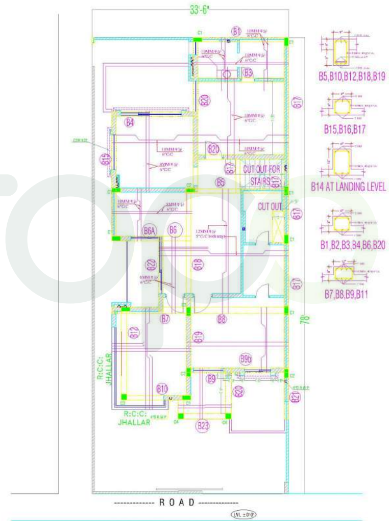
First Floor Slab Structure Plan
