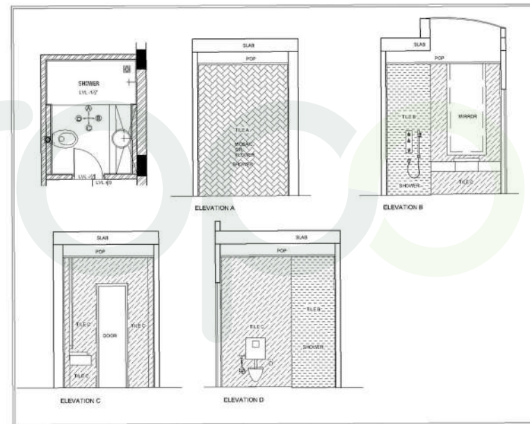
Master Toilet First Floor
