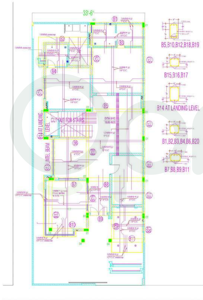
Ground Floor Slab Structure Plan
