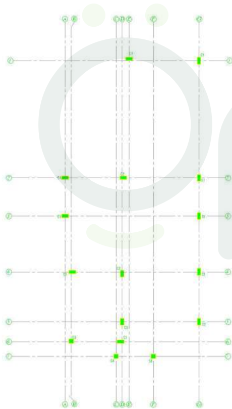
Column Grid Plan
