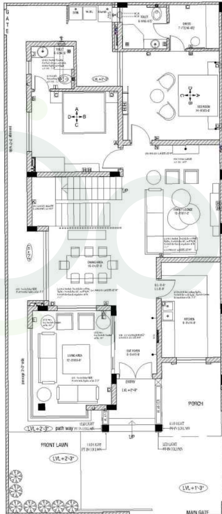
Ground Floor Electrical
