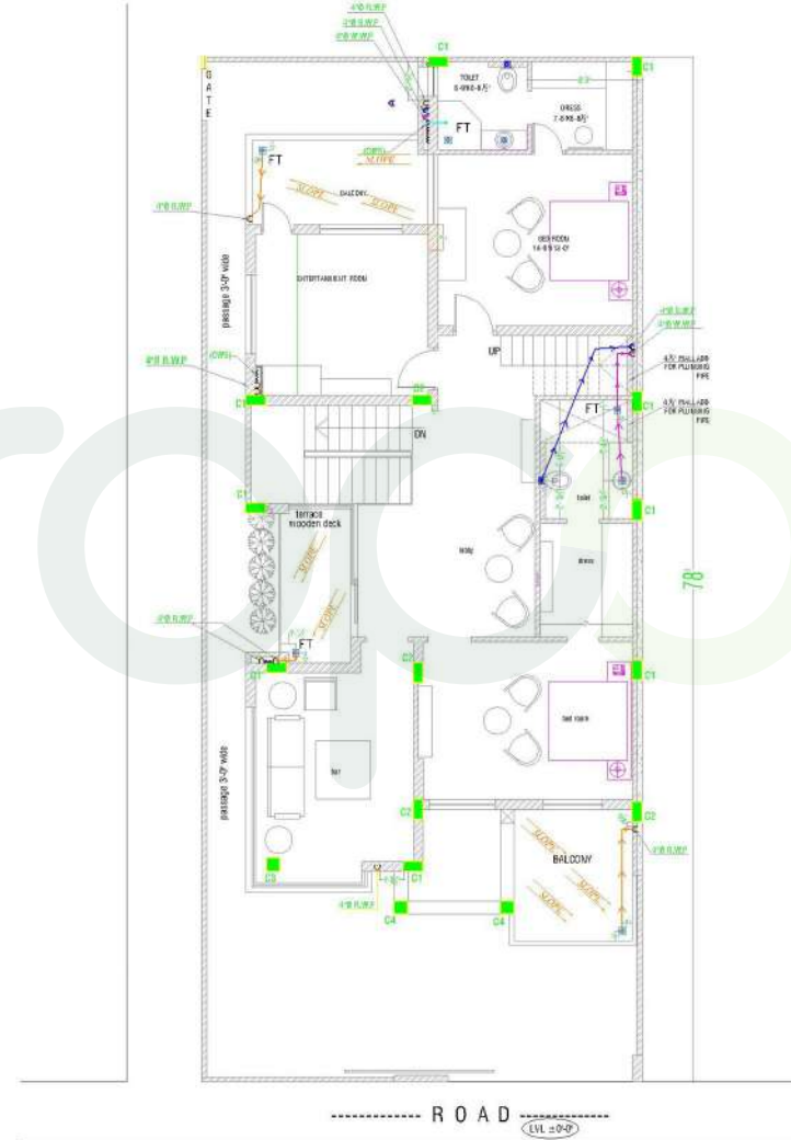
First Floor Plumbing Plan
