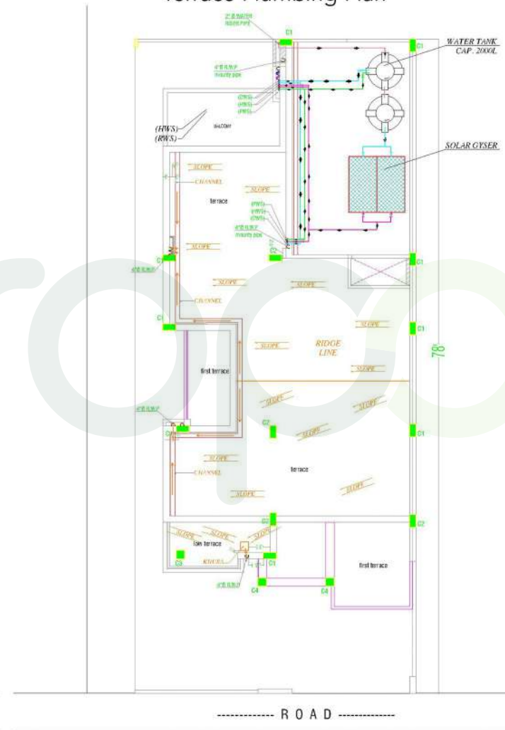
Terrace Plumbing Plan
