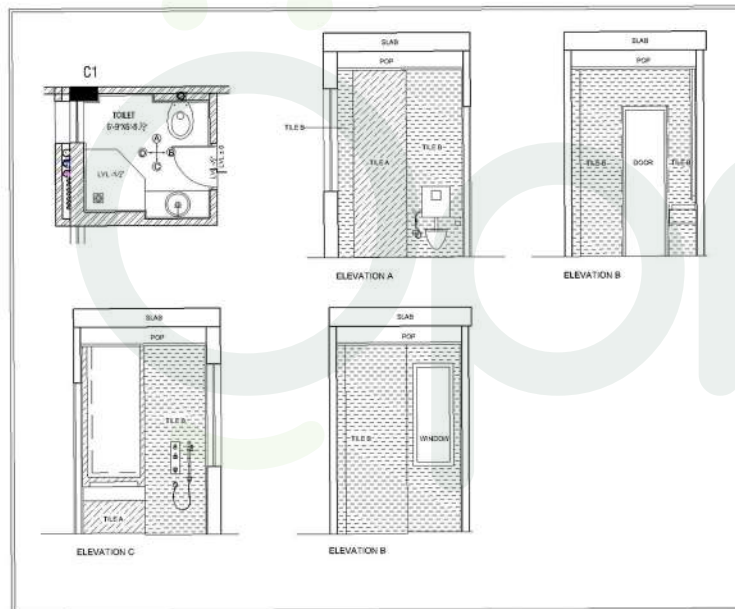
Master Toilet Ground Floor
